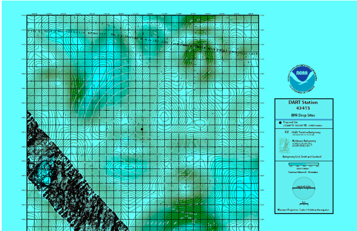
Siting Diagram Station 43413
