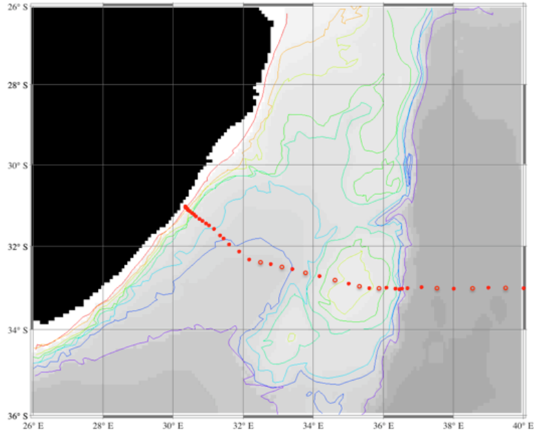
R/V Roger Reville CO2/CLIVAR I5, March 2009 – detail of intended CTD/rosette station positions, prepared for the South African clearance request by James Swift (UCSD/SIO). Solid circles are repeats of the 2002 stations along the I5 track. Open circles are optional stations.
